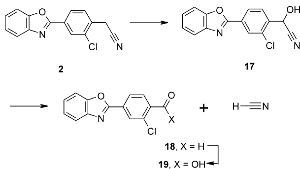
Scheme 4. Proposed major metabolite in rat PK study.
