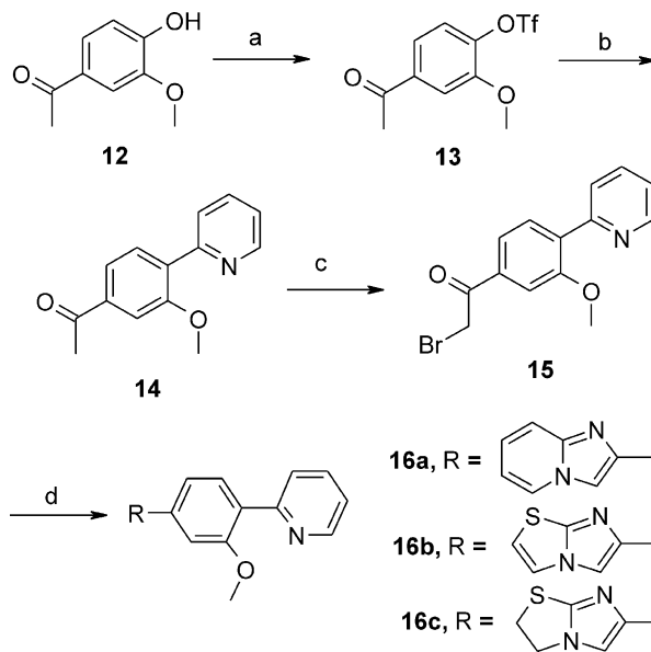
Scheme 3. Reagents: (a) Cs 2 CO 3 , N -phenyltrifluoromethanesulfonimide, DMF; (b) 2-pyridyl zinc bromide, Pd(PPh 3 ) 4 , THF; (c) Br 2 , AcOH/HBr; (d) 16a : 2-aminopyridine, EtOH; 16b : 2-aminothiazole, EtOH; 16c : 2-amino-2-thiazoline, EtOH.
