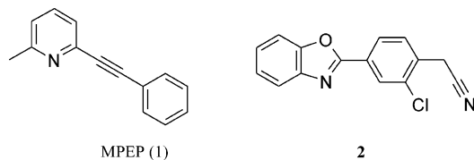
Figure 1. mGluR5 antagonists.
