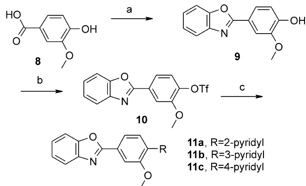
Scheme 2. Reagents: (a) 2-aminophenol, trimethylsilylpolyphosphate; (b) Cs 2 CO 3 , N -phenyltrifluoromethanesulfonimide, DMF; (c) 11a : 2- tri-n -butylstannylpyridine, Pd(PPh 3 ) 4 , DMF; 11b : 3-pyridylboronic acid, Pd(PPh 3 ) 4 , K 2 CO 3 , n -Bu 4 NBr, DMF/H 2 O; 11c : 4-pyridylboronic acid, Pd(PPh 3 ) 4 , K 2 CO 3 , n -Bu 4 NBr, DMF/H 2 O.
